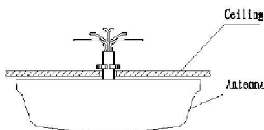
Installation Sketch
